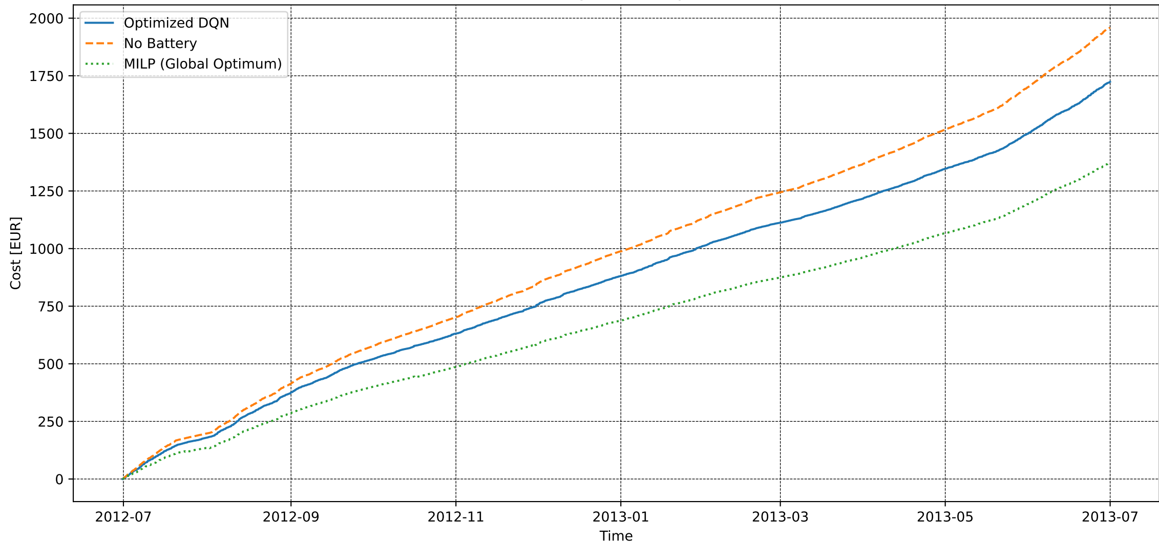
User 148 - Basic Training - Electricity Cost [DQN vs MILP]
